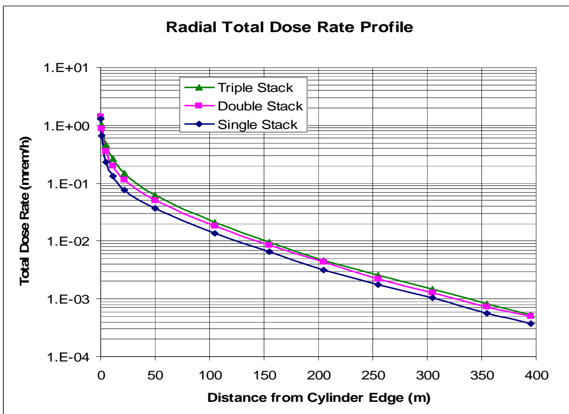
Figure 6-8 Radial Total Dose Rate Profile for 30x30 Array
